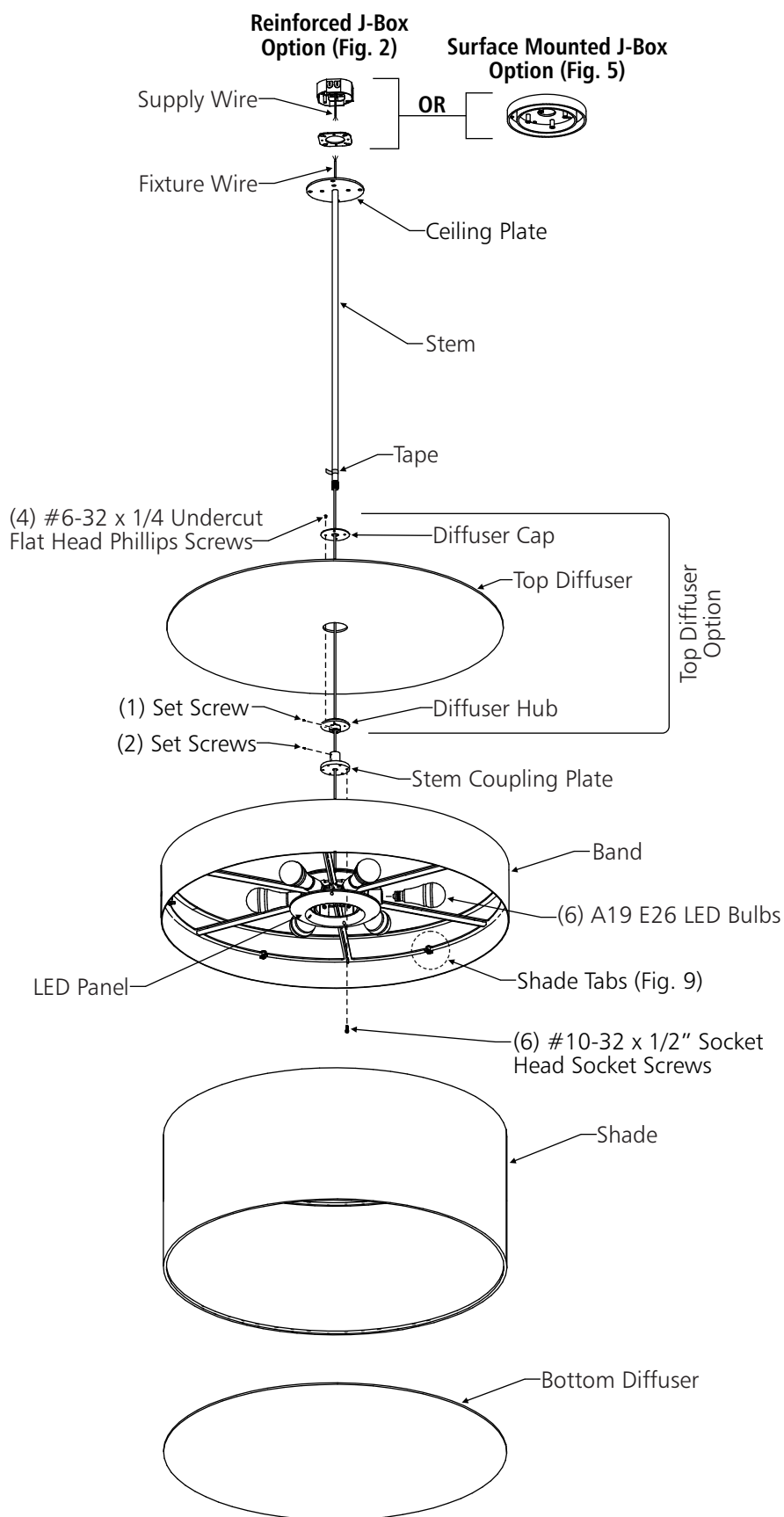
Fig.1 - Fixture Components
